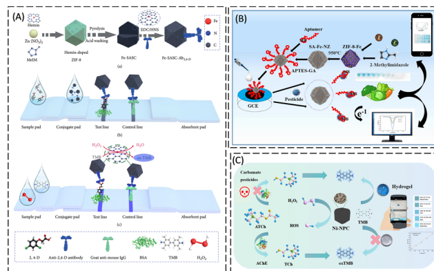
Fig. 5 (A) Schematics showing Fe-SASC synthesis, antibody conjugation (Fe-SASC-Ab 2,4-D ) and the Fe-SASC-based lateral-flow immunoassay strip for 2,4-D detection, reproduced with permission from ref. 100, Copyright 2022, AAAS, (B) a scheme showing the assembly and detection process of the SA-Fe SANs dual-mode biosensor, reproduced with permission from ref. 101, Copyright 2024, Elsevier B.V., and (C) Ni-NPC SANs platform for carbamate pesticide remediation and smartphone visualization, reproduced with permission from ref. 103, Copyright 2024, American Chemical Society.
