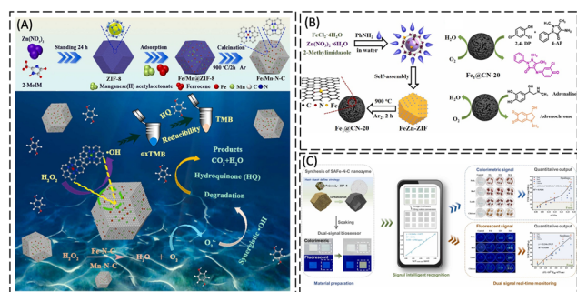
Fig. 4 (A) Synthetic route for Fe/Mn co-doped N-C SANs and integrated platform demonstrating hydroquinone quantification through colorimetric analysis coupled with oxidative degradation, reproduced with permission from ref. 93, Copyright 2023, Elsevier B.V., (B) preparation scheme for Fe 1 @CN-20 SANs and their applications in simultaneous detection and degradation of 2,4-DP and adrenaline pollutants, reproduced with permission from ref. 94, Copyright 2022, Elsevier B.V., and (C) portable colorimetric-fluorescence dual-signal biosensor for visual detection of VA, reproduced with permission from ref. 96, Copyright 2023, Elsevier B.V.
