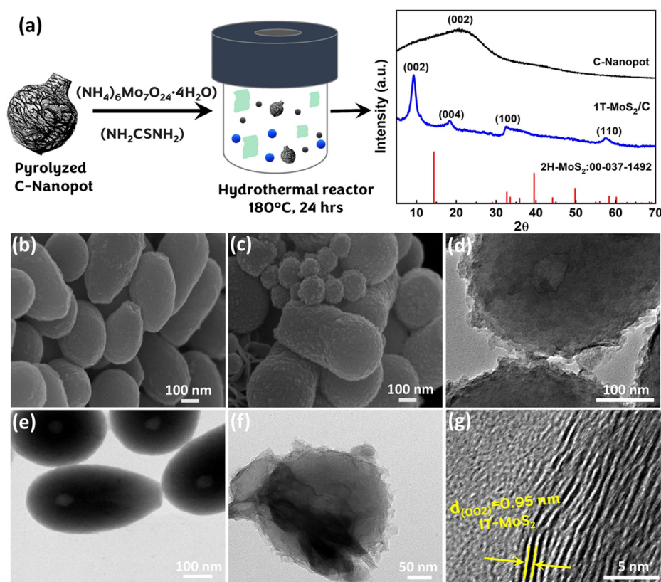
Fig. 1 (a) Schematic showing the synthesis of 1T MoS 2 on carbon nanopots (1T MoS 2 /C) (left panel) and XRD (right panel); (b and e) SEM and TEM micrographs of the pyrolyzed carbon nanopots, respectively; (c) SEM of 1T MoS 2 /C; (d and f)-TEM of 1T MoS 2 /C; (g) high-resolution TEM image showing diffraction fringes of 1T MoS 2 .
