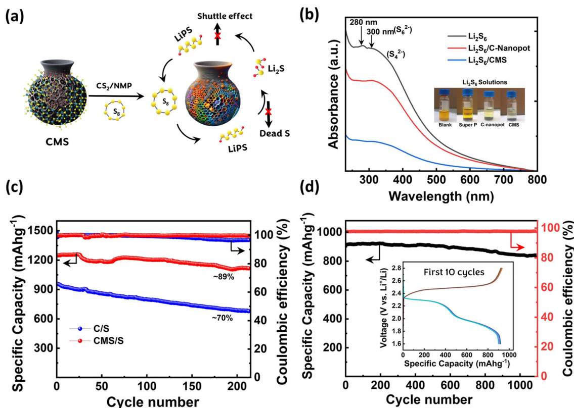
Fig. 6 (a) Sulfur-loaded CMS (CMS/S) sample showing the mechanism of electrocatalytic conversion of polysulfides. (b) Polysulfide adsorption test and UV visible spectra of a polysulfides-saturated samples. (c) Specific capacity retention and coulombic efficiencies of the C/S and CMS/S electrodes obtained at a low current density of 0.2 \text{ A g}^{-1} . (d) Cyclic stability and coulombic efficiency of CMS/S at 1 \text{ A g}^{-1} (inset shows initial ten charge–discharge cycles).
