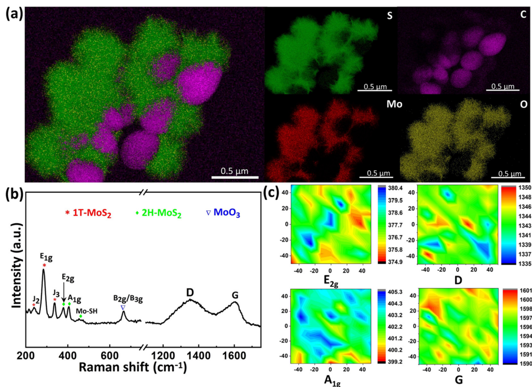
Fig. 4 (a) Elemental micrographs of the CMS sample showing the S, C, Mo, and O maps; (b) Raman spectrum of CMS; (c) Raman mapping data for MoS_2 ( E_{2g} and A_{1g} ) and carbon (D and G peaks) in CMS.
