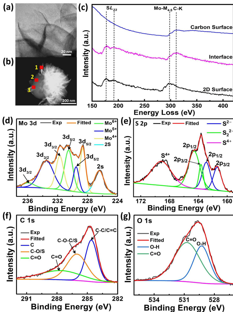
Fig. 3 (a) TEM image showing the MoS 2 layers; (b) STEM micrograph showing various EELS data acquisition points on the CMS sample marked in 1, 2 and 3; (c) EELS spectra obtained on three different regions of the sample. High-resolution XPS spectra of CMS: (d) Mo 3d, (e) S 2p, (f) C 1s, and (g) O 1s.
