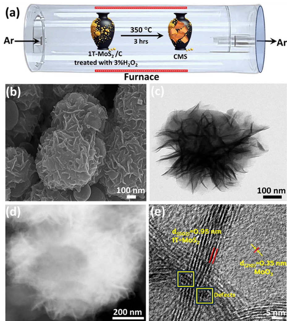
Fig. 2 (a) Scheme illustrating the synthesis of CMS; (b) SEM of CMS; (c) TEM of CMS (d) STEM of CMS; (e) HR-TEM of CMS.
