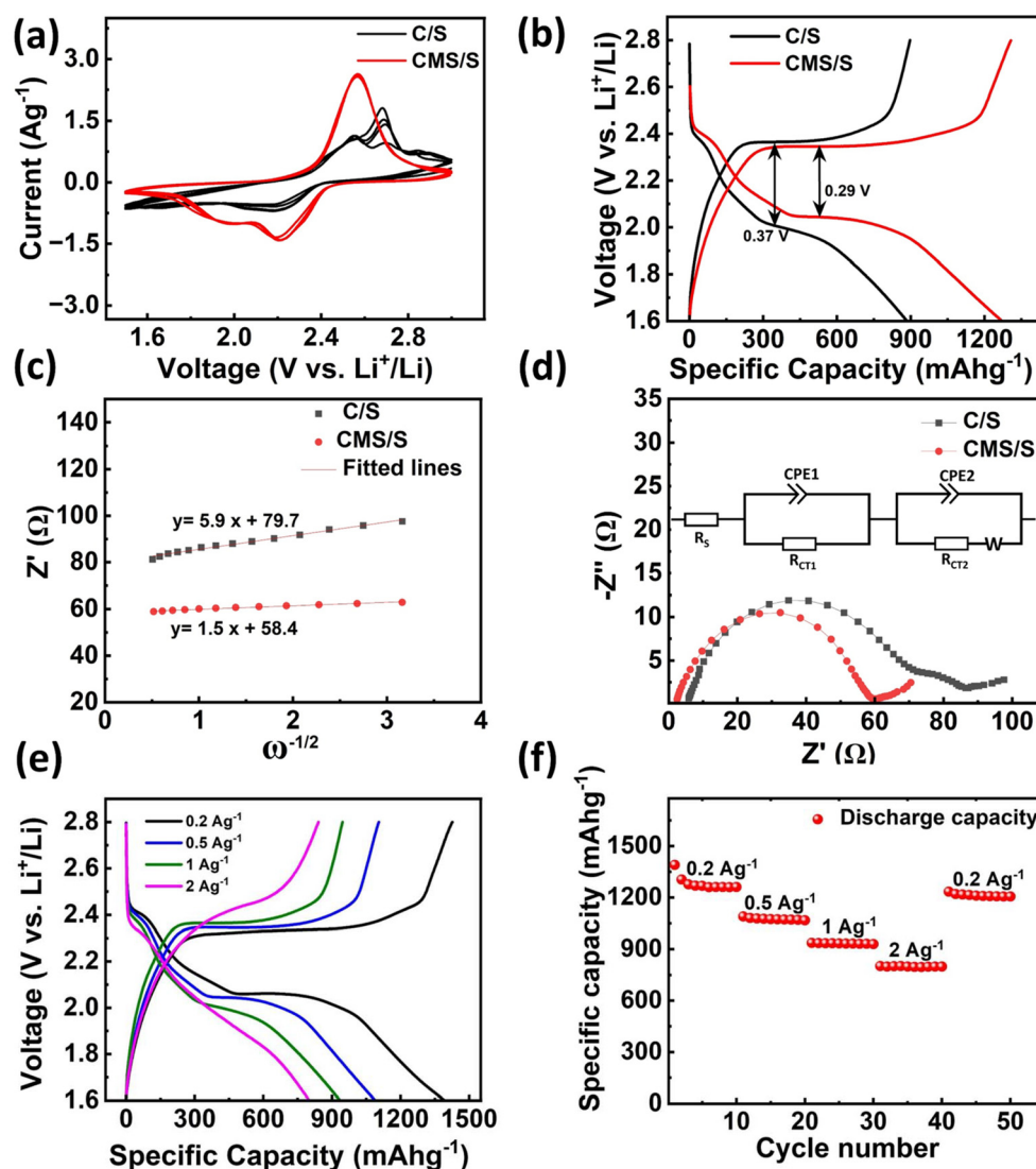
Fig. 5 (a) Comparison of the cyclic voltammetric response of C/S and CMS/S. (b) Comparative galvanostatic charge–discharge profiles. (c) Warburg slopes determination from the Z' vs. \omega^{-1/2} plot; (d) EIS plot. (e) Initial specific capacities of CMS/S obtained at various current densities. (f) Rate capability of the CMS/S obtained from 0.2 A g -1 to 2 A g -1 .
