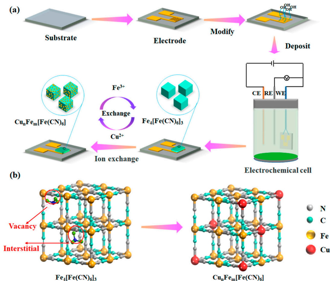
Figure 12. (a) Stepwise fabrication of the Cu–Fe PBA-based capacitive sensor on Au interdigitated electrodes (IDEs), including surface modification, PB film deposition, and ion-exchange to form Cu–Fe PBAs. (b) Crystal structures of PB and Cu–Fe PBAs, highlighting adsorption sites for ammonia gas. Reproduced with permission from ACS [182].
