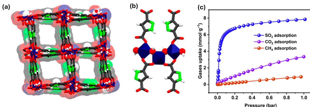
Figure 9. (a) Structure of MOF-303: view along the channel c-axis and (b) metal cluster and linker arrangement along the b-axis. Atoms are labeled as follows: blue, \text{AlO}_4(\mu\text{-OH})_2 octahedra; gray, carbon; white, hydrogen; green, nitrogen; red, oxygen. (c) Single-component adsorption isotherms of \text{SO}_2 (blue), \text{CO}_2 (purple), and \text{CH}_4 (red) at 298 K and 1 bar. Reproduced with permission from ACS [124].
