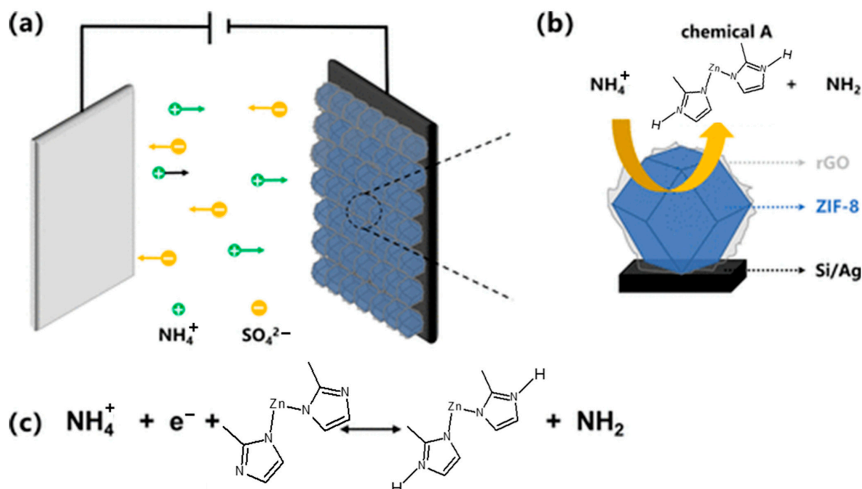
Figure 11. (a) Schematic of the DPV-based detection setup. (b) Enlarged view of the ZIF-8/rGO working electrode from (a). (c) Chemical reaction occurring during \text{NH}_4^+ detection. Reproduced with permission from ACS [161].
