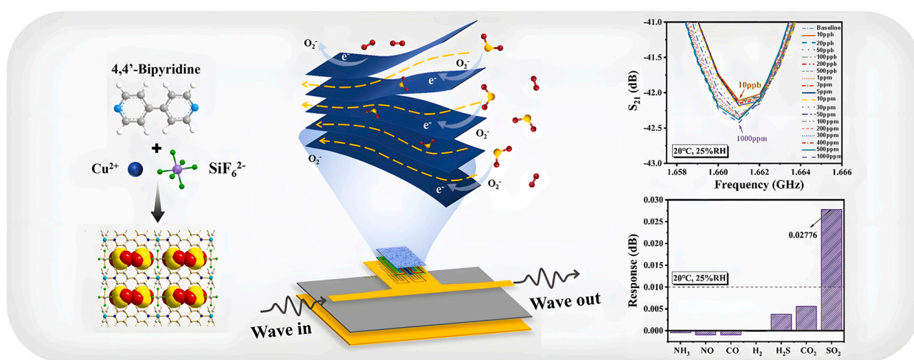
Figure 10. Illustration of the SIFSIX-1-Cu microwave gas sensor for SO 2 detection, where adsorption in the MOF's nanochannels induces changes in electromagnetic properties, allowing sensitive, selective, and moisture-tolerant detection at ambient conditions. Reproduced with permission from Elsevier [141].
