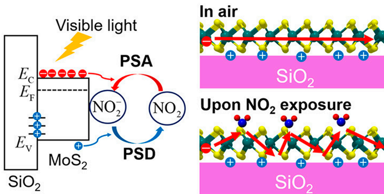
Figure 4. Schematic illustration of the electrochemical mechanism of \text{NO}_2 gas sensing on a \text{MoS}_2 -based field-effect transistor (FET) sensor. Upon illumination, photoexcited charge carriers are generated in the \text{MoS}_2 channel. Reproduced with permission from ACS [87].
