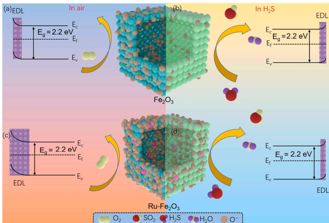
Figure 5. Schematic of the gas-sensing mechanism of Fe 2 O 3 and Ru-Fe 2 O 3 hollow-box sensors. (a,c) In air, oxygen adsorbs and ionizes on the surface, capturing electrons and forming an electron depletion layer (EDL), increasing resistance. (b,d) Exposure to reducing gases reacts with adsorbed oxygen, releasing electrons, thinning the EDL, and decreasing resistance. Reproduced with permission from Elsevier [98].
