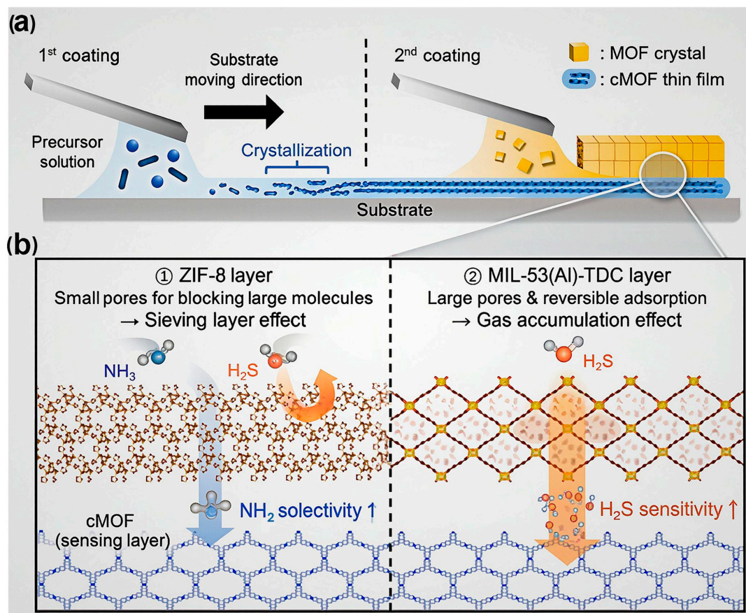
Figure 6. Schematic illustration of (a) the stepwise fabrication of layered MOF-on-cMOF films via the solution-shearing technique and (b) the synergistic roles of the conductive and porous MOF layers in enhancing gas adsorption, charge transport, and overall sensing performance. Reproduced with permission from ACS [99].
