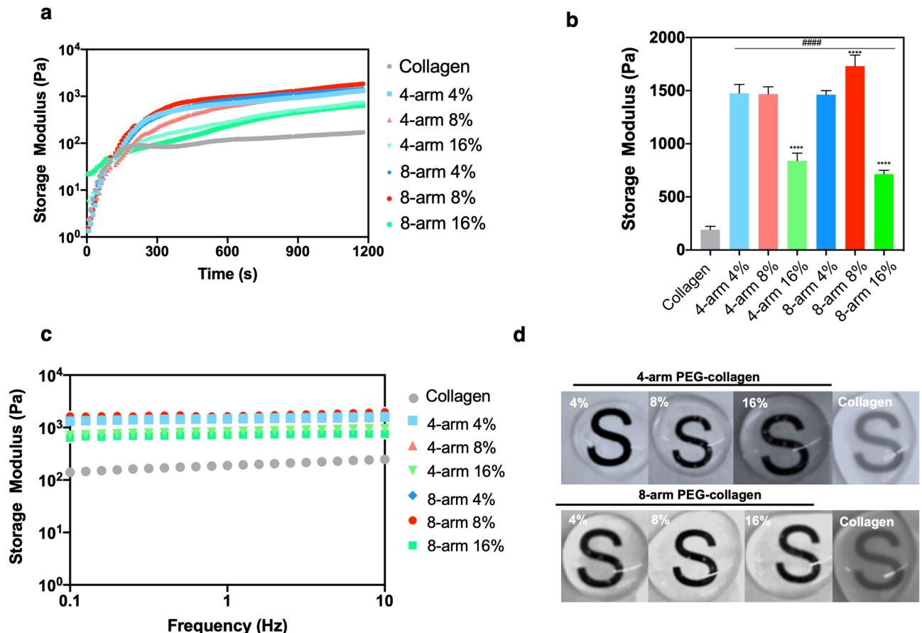
Figure 2. Physical properties of chemically crosslinked PEG-collagen hydrogels by NHS chemistry and non-crosslinked (physical) collagen hydrogels. (a) Dynamic moduli of 4-arm PEG-collagen and 8-arm PEG-collagen hydrogels using different concentrations of PEG polymer as function of time during gelation. The hydrogels were mounted immediately after mixing. (b) Dynamic moduli of 4-arm PEG-collagen and 8-arm PEG-collagen hydrogels at different concentrations of PEG polymer. 4 and 8-arm PEG-collagen at 16% v/v PEG show lower storage modulus (**** p < 0.0001 ) compared to 4 and 8-arm PEG-collagen at 4 and 8%. 8-arm PEG-collagen hydrogel at 8% showed higher storage modulus (**** p < 0.0001 ) compared to all other PEG concentrations and type. Collagen crosslinked with 4 and 8-arm PEG polymer at all concentrations showed significant higher storage modulus (#### p < 0.0001 ) compared to non-crosslinked collagen hydrogel; data is presented as mean \pm SD, two-way ANOVA ( p < 0.005 ) was used to detect statistical differences followed by Tukey's multiple comparisons test. (c) Dynamic moduli of 4-arm PEG-collagen and 8-arm PEG-collagen hydrogels as a function of frequency. (d) Photographs of 4 and 8-arm PEG-collagen and non-crosslinked (physical) collagen hydrogels.
