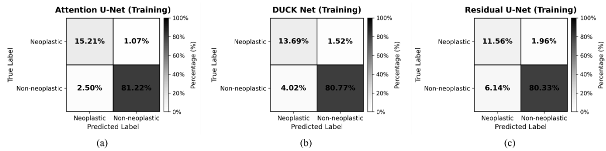
Figure 2. Mean confusion matrix of fivefold cross-validation in the training cohort.
