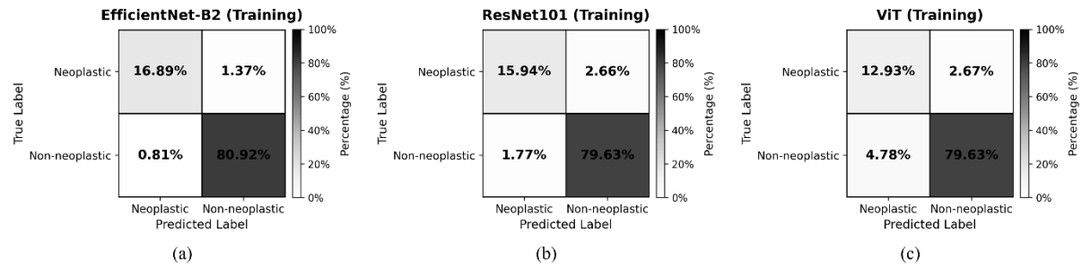
Figure 5. Mean confusion matrix of fivefold cross-validation in the training cohort.
