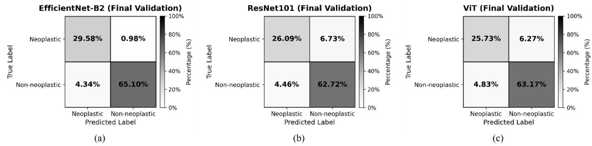
Figure 7. Mean confusion matrix of fivefold cross-validation in the final validation cohort.
